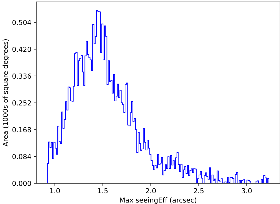
internal_u_expt38_nscale1.0v3.4_10yrs Yr 1 u band: Max seeingEff
