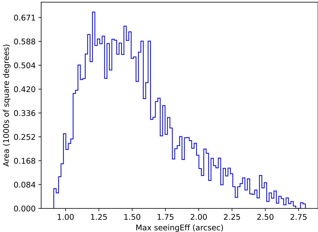
internal_u_expt38_nscale1.0v3.4_10yrs Yr 1 g band: Max seeingEff
