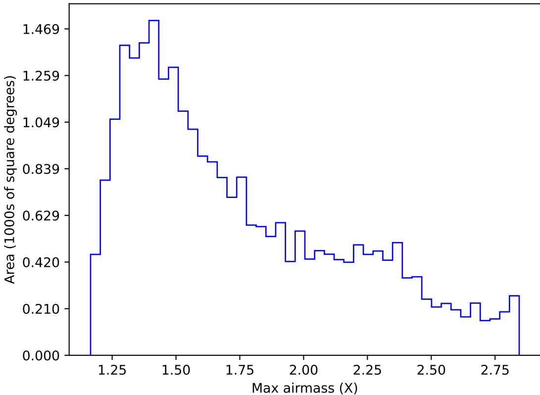
internal_u_expt38_nscale1.0v3.4_10yrs Yr 1 z band: Max airmass
