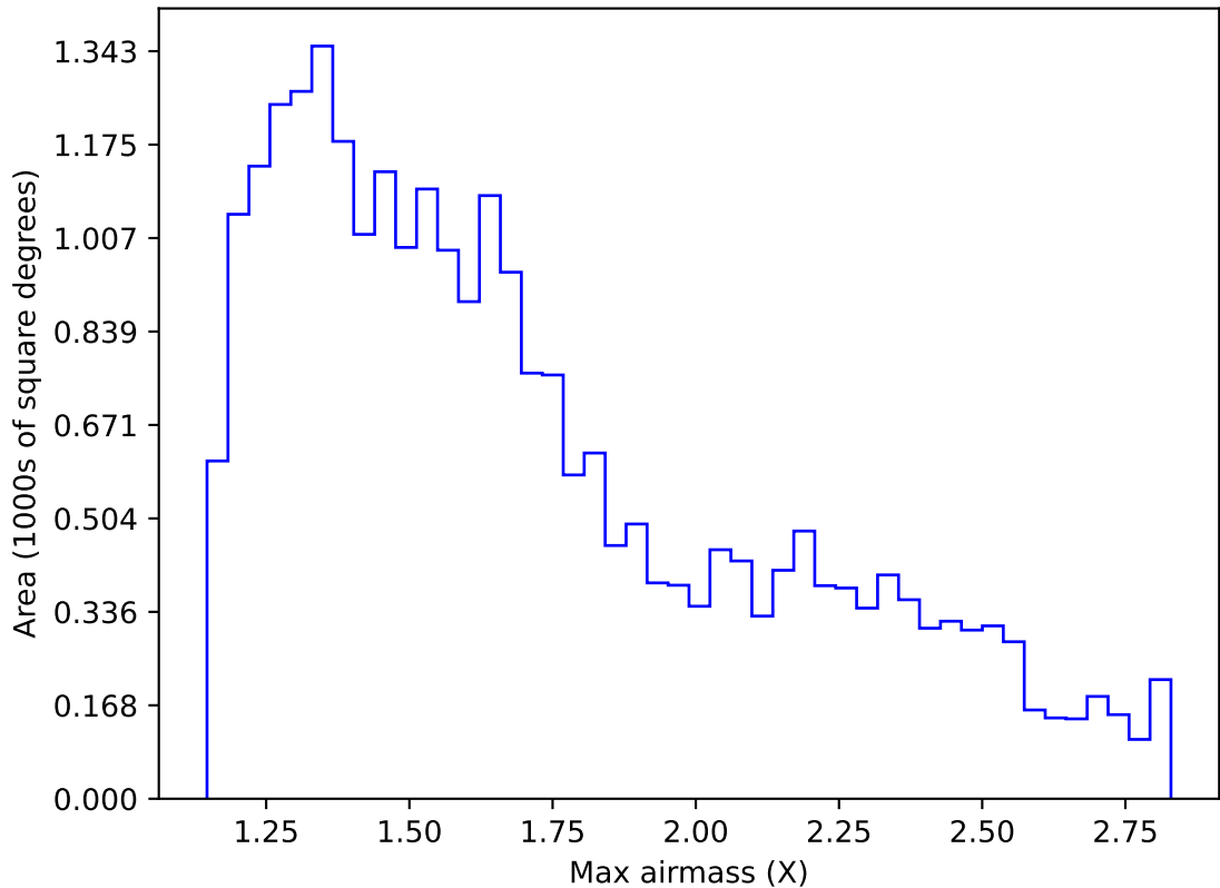
internal_u_expt38_nscale1.0v3.4_10yrs Yr 1 i band: Max airmass
