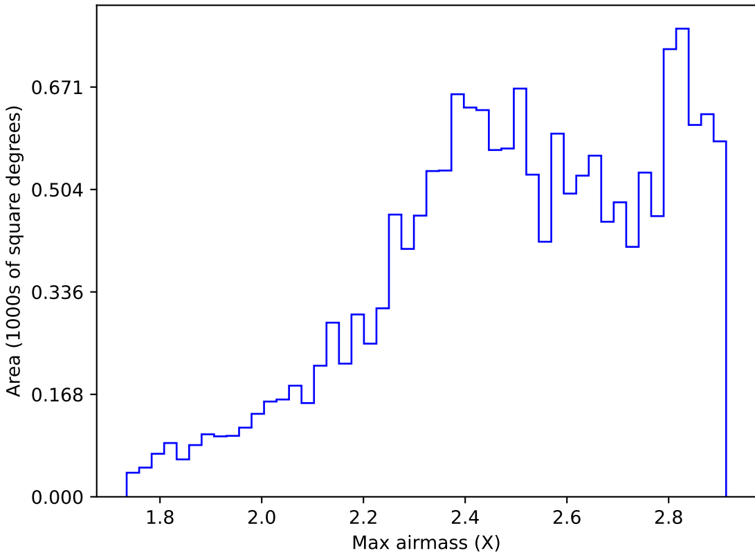
internal_u_expt38_nscale1.0v3.4_10yrs WFD z band: Max airmass
