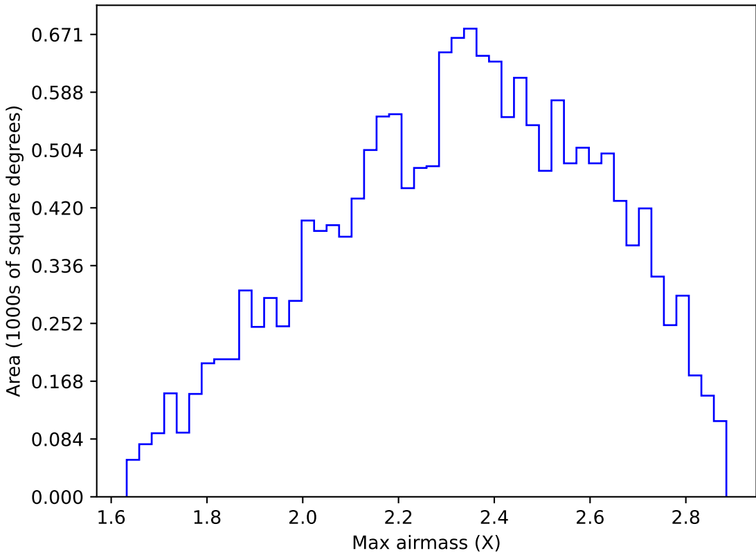
internal_u_expt38_nscale1.0v3.4_10yrs WFD y band: Max airmass
