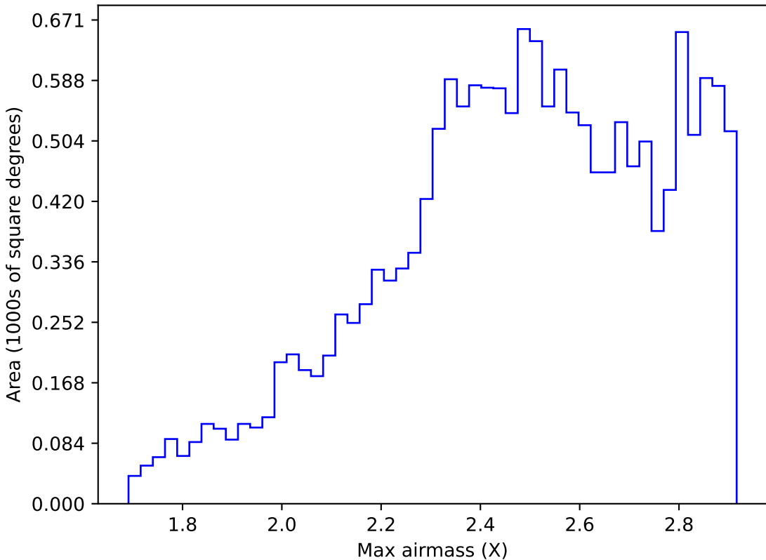
internal_u_expt38_nscale1.0v3.4_10yrs WFD i band: Max airmass
