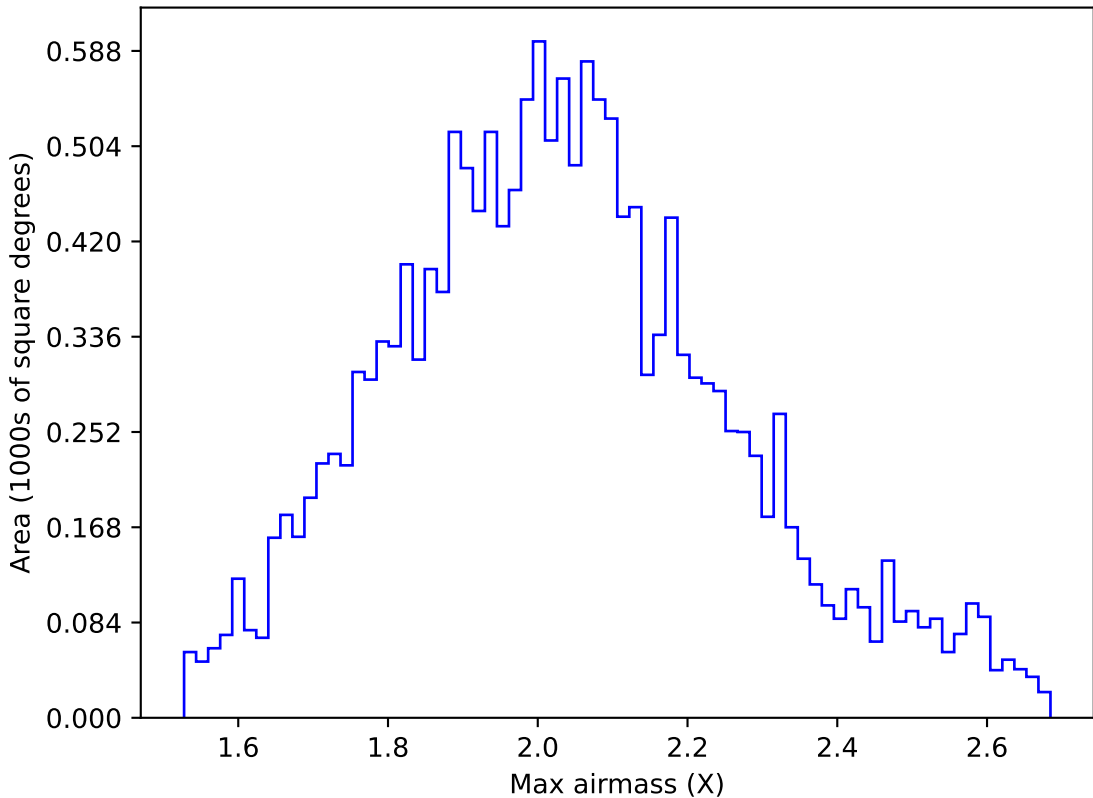
internal_u_expt38_nscale1.0v3.4_10yrs WFD g band: Max airmass
