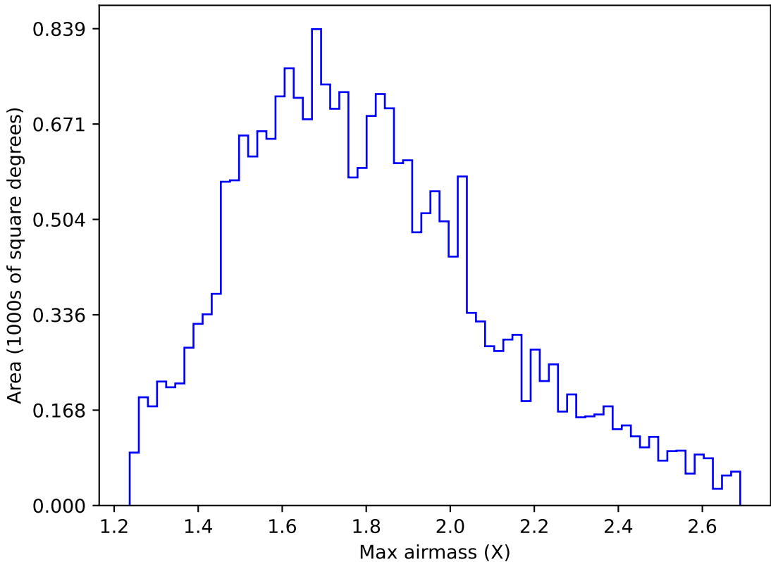
internal_u_expt38_nscale1.0v3.4_10yrs All sky u band: Max airmass
