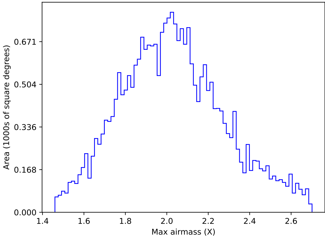
internal_u_expt38_nscale1.0v3.4_10yrs All sky g band: Max airmass
