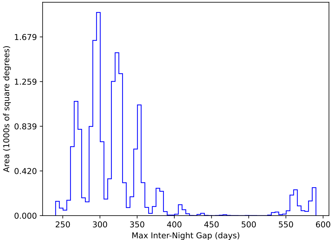
internal_u_expt38_nscale1.0v3.4_10yrs WFD y band: Max Inter-Night Gap
