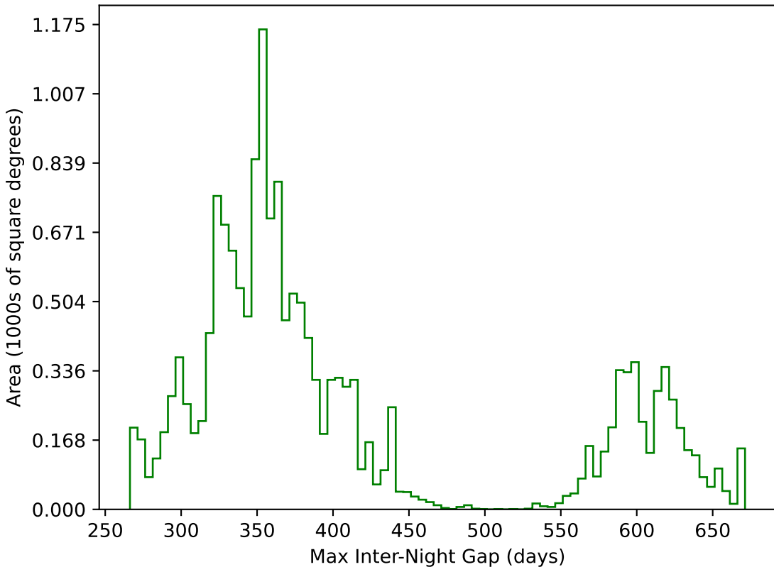
internal_u_expt38_nscale1.0v3.4_10yrs WFD g band: Max Inter-Night Gap
