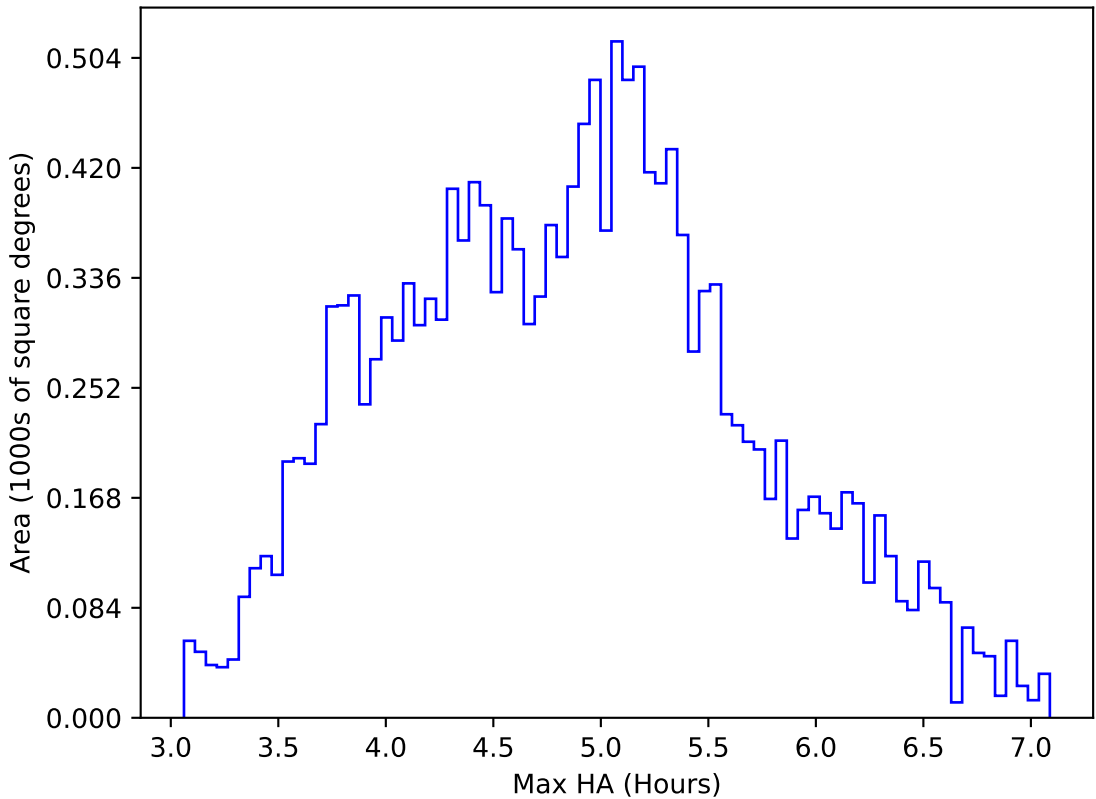
internal_u_expt38_nscale1.0v3.4_10yrs WFD i band: Max HA
