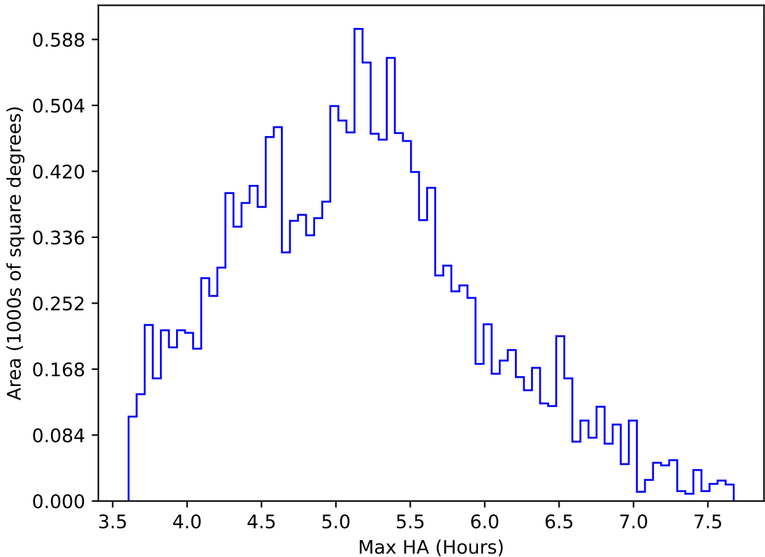
internal_u_expt38_nscale1.0v3.4_10yrs WFD all bands: Max HA
