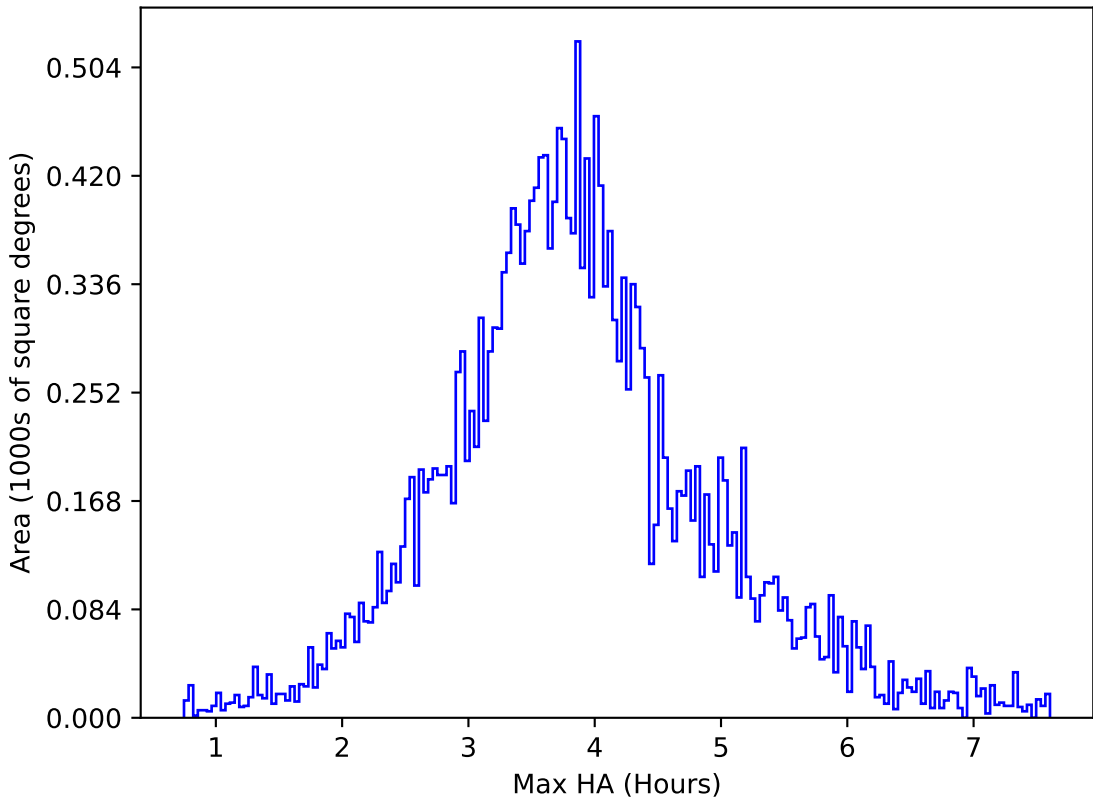
internal_u_expt38_nscale1.0v3.4_10yrs All sky u band: Max HA
