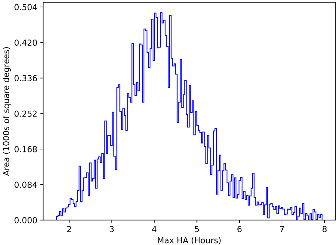
internal_u_expt38_nscale1.0v3.4_10yrs All sky r band: Max HA
