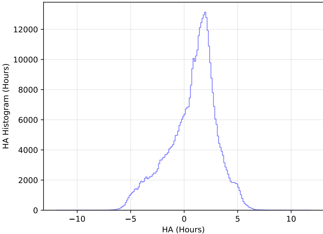
internal_u_expt38_nscale1.0v3.4_10yrs WFD z band: HA Histogram
