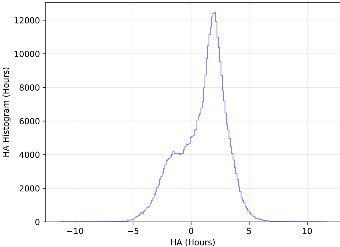
internal_u_expt38_nscale1.0v3.4_10yrs WFD y band: HA Histogram
