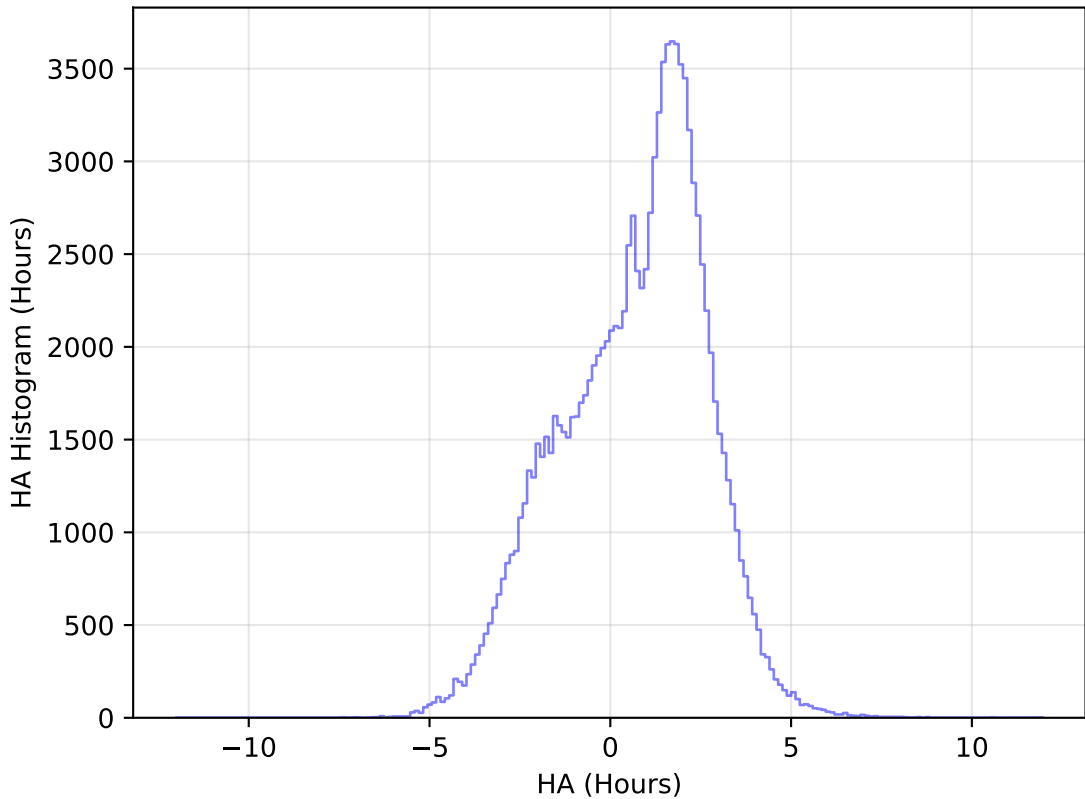
internal_u_expt38_nscale1.0v3.4_10yrs WFD u band: HA Histogram
