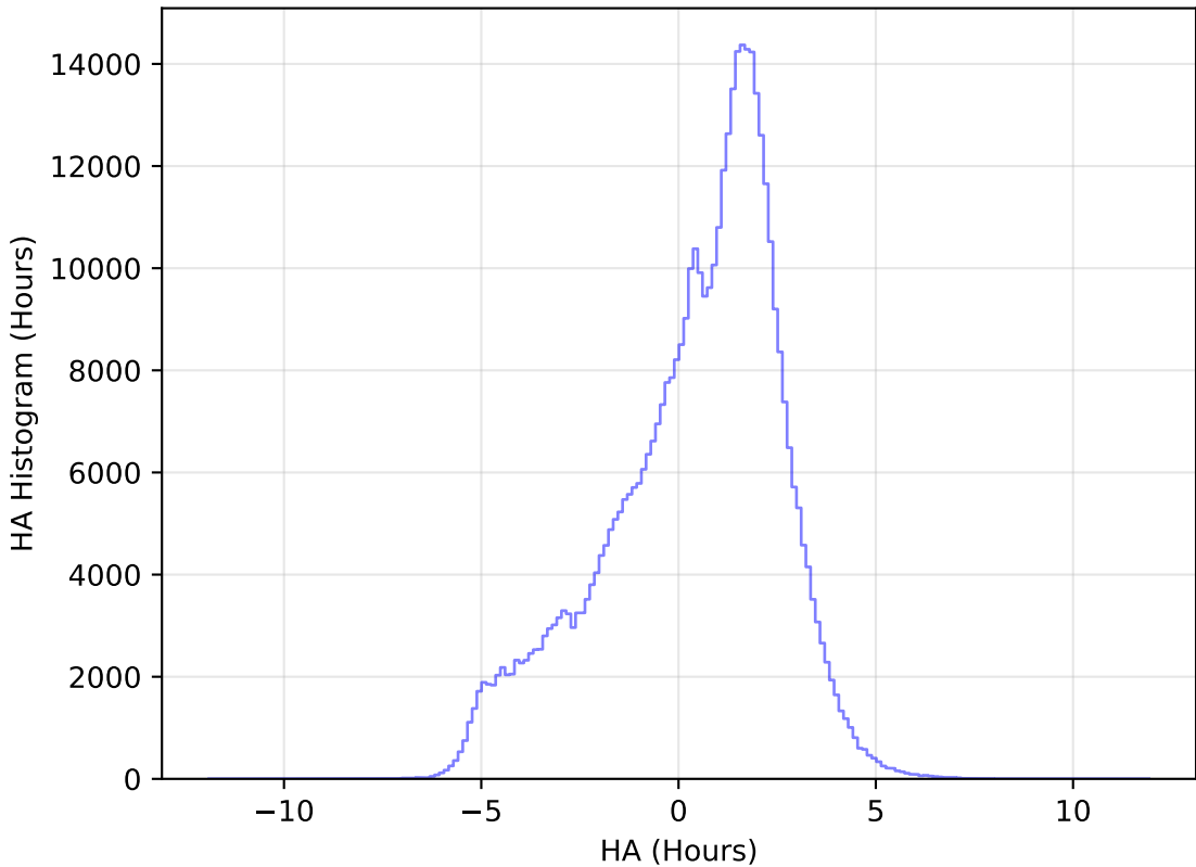
internal_u_expt38_nscale1.0v3.4_10yrs WFD r band: HA Histogram
