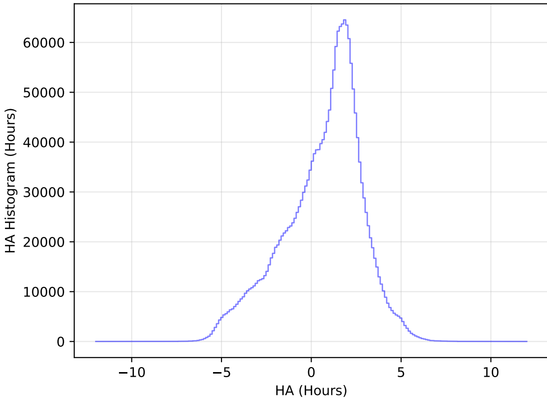
internal_u_expt38_nscale1.0v3.4_10yrs WFD all bands: HA Histogram
