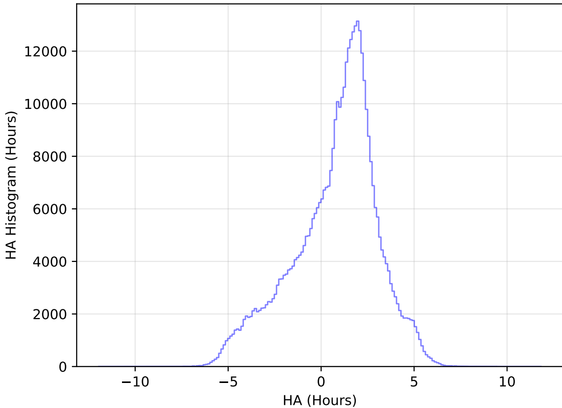
internal_u_expt38_nscale1.0v3.4_10yrs All sky z band: HA Histogram
