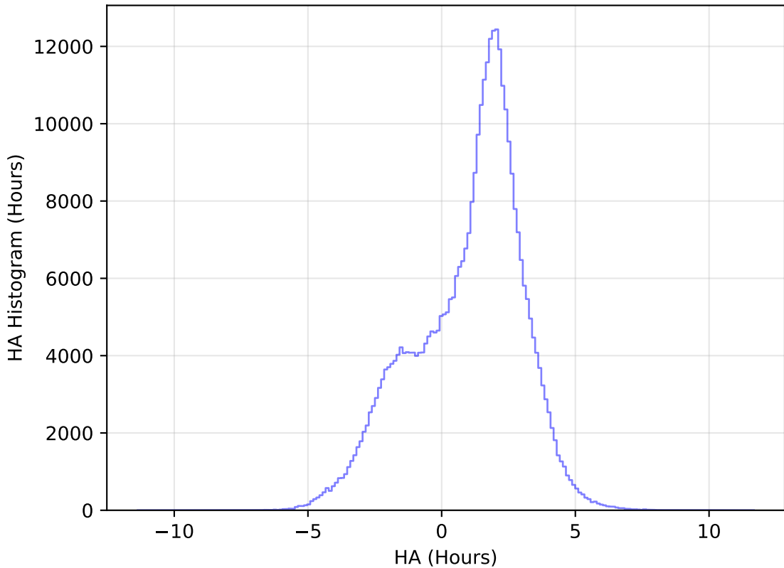
internal_u_expt38_nscale1.0v3.4_10yrs All sky y band: HA Histogram
