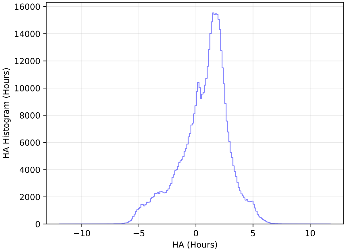
internal_u_expt38_nscale1.0v3.4_10yrs All sky i band: HA Histogram
