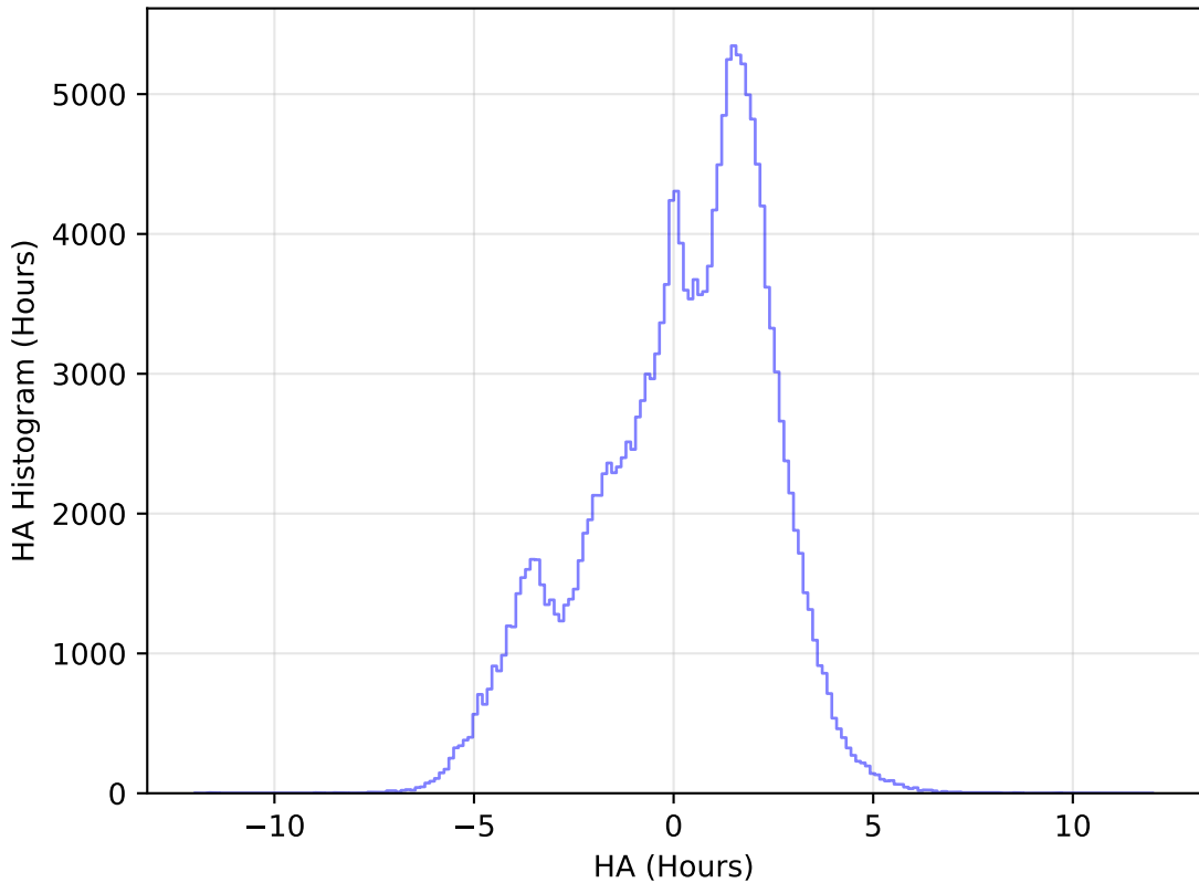
internal_u_expt38_nscale1.0v3.4_10yrs All sky g band: HA Histogram
