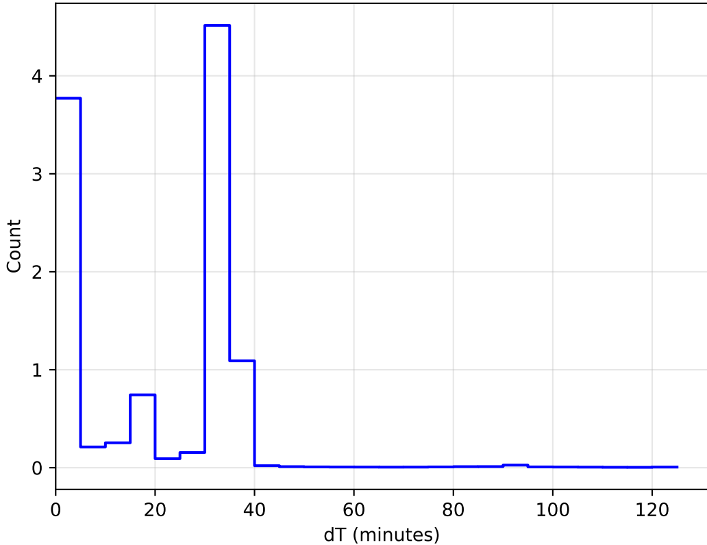
internal_u_expt38_nscale1.0v3.4_10yrs WFD: DeltaT Histogram
