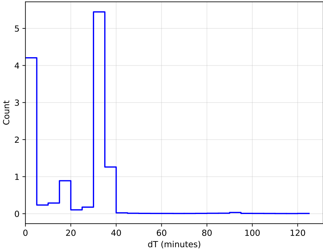
internal_u_expt38_nscale1.0v3.4_10yrs All sky: DeltaT Histogram
