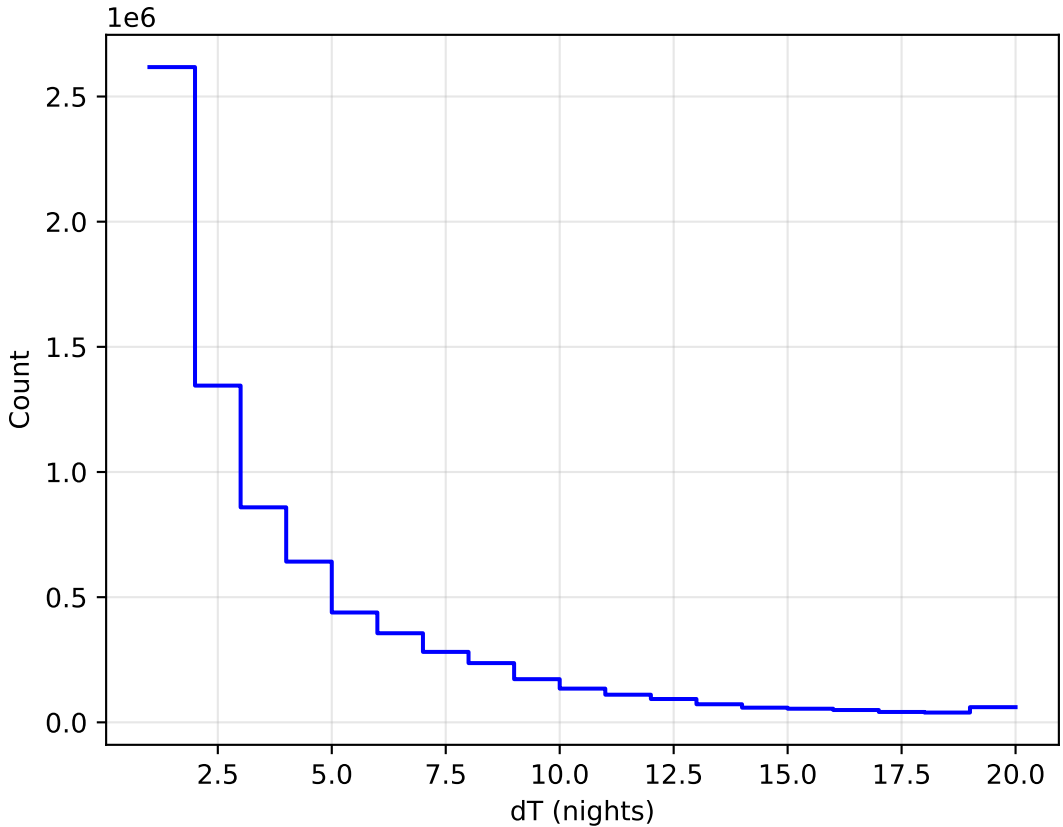
internal_u_expt38_nscale1.0v3.4_10yrs WFD all bands: DeltaNight Histogram
