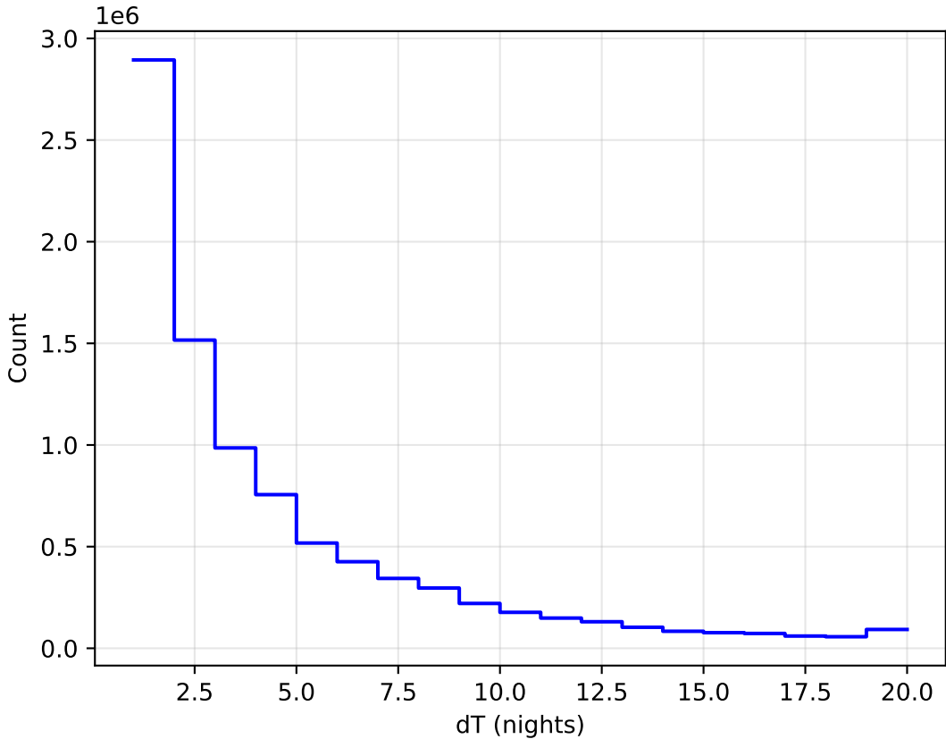
internal_u_expt38_nscale1.0v3.4_10yrs All sky all bands: DeltaNight Histogram
