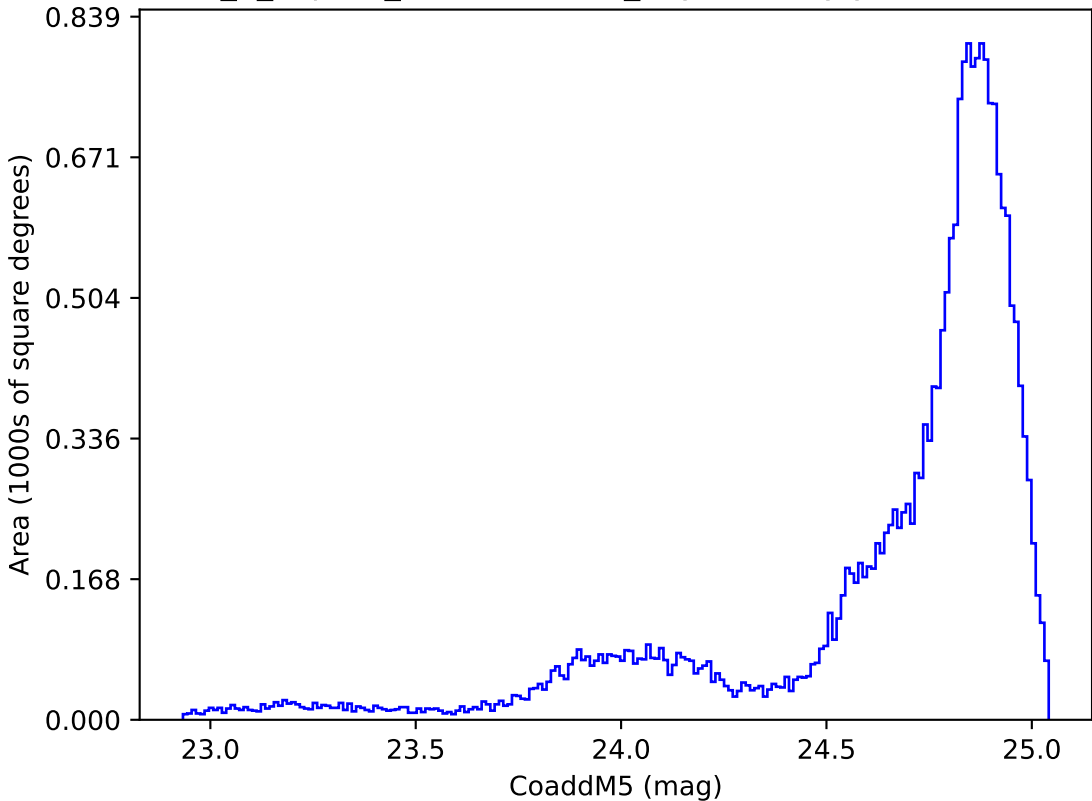
internal_u_expt38_nscale1.0v3.4_10yrs All sky y band: CoaddM5
