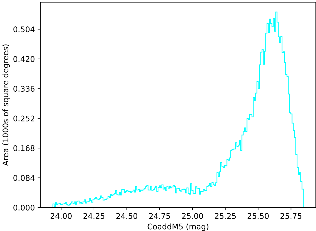
internal_u_expt38_nscale1.0v3.4_10yrs All sky u band: CoaddM5
