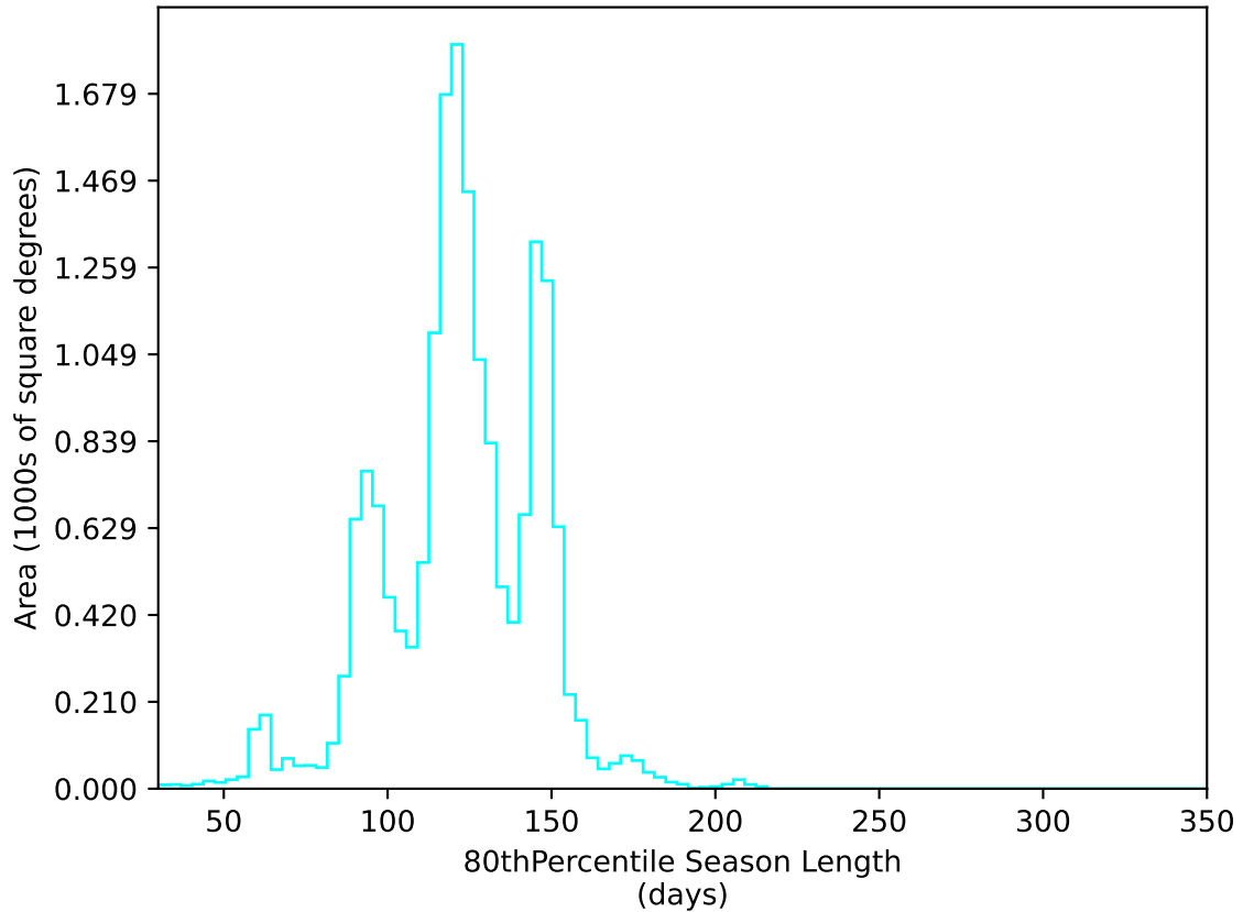
internal_u_expt38_nscale1.0v3.4_10yrs WFD u band: 80thPercentile Season Length
