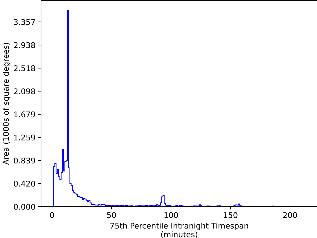
internal_u_expt38_nscale1.0v3.4_10yrs WFD i band: 75th Percentile Intranight Timespan
