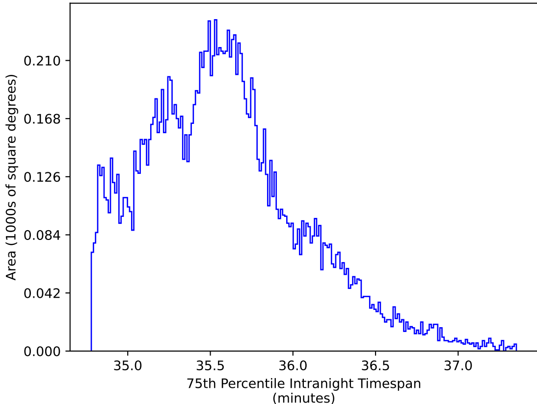
internal_u_expt38_nscale1.0v3.4_10yrs WFD all bands: 75th Percentile Intranight Timespan
