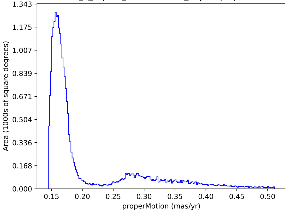
internal_u_expt38_nscale1.0v3.4_10yrs : properMotion
