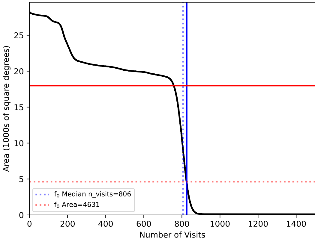
internal_u_expt38_nscale1.0v3.4_10yrs : fO
