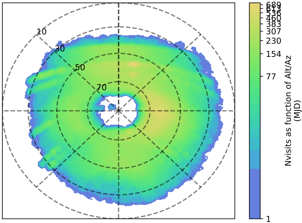
internal_u_expt38_nscale1.0v3.4_10yrs u: Nvisits as function of Alt/Az
