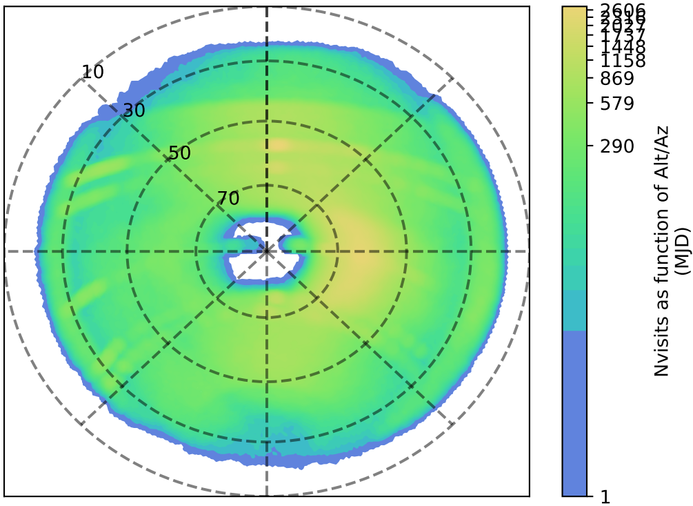
internal_u_expt38_nscale1.0v3.4_10yrs i: Nvisits as function of Alt/Az
