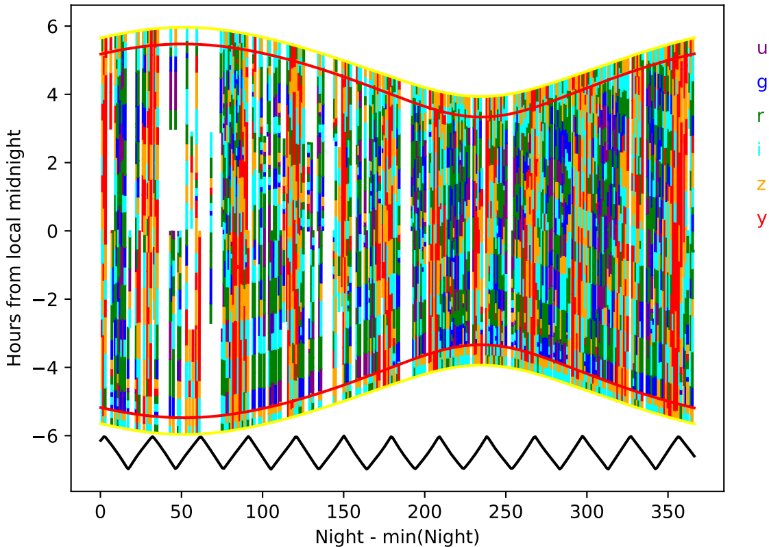
internal_u_expt38_nscale1.0v3.4_10yrs year 9-10: Hourglass
