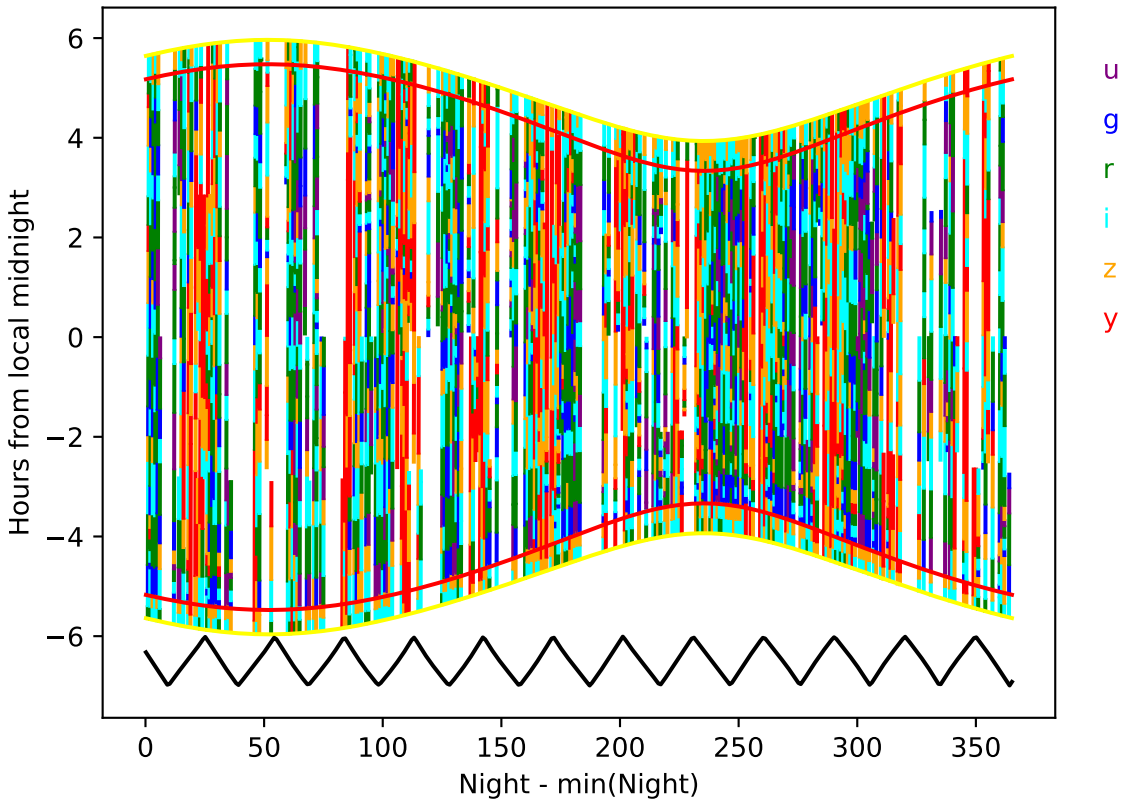
internal_u_expt38_nscale1.0v3.4_10yrs year 7-8: Hourglass
