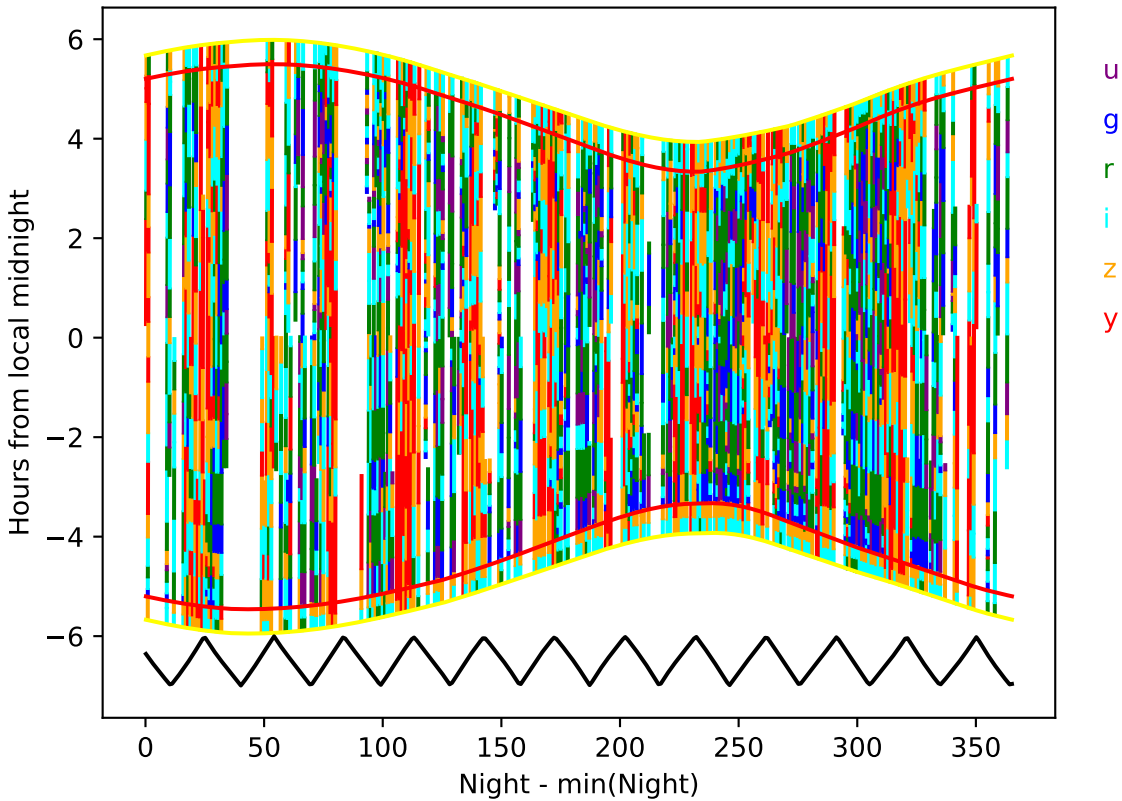
internal_u_expt38_nscale1.0v3.4_10yrs year 4-5: Hourglass
