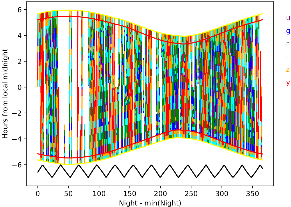
internal_u_expt38_nscale1.0v3.4_10yrs year 3-4: Hourglass
