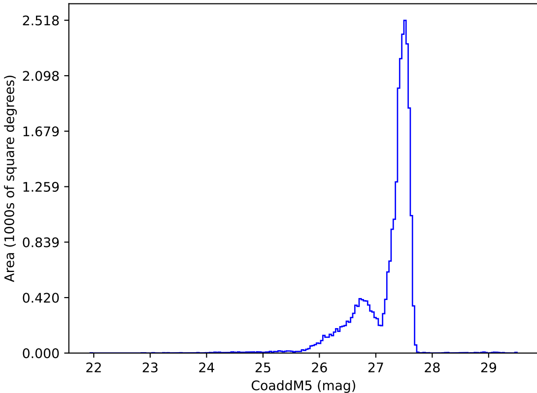
internal_u_expt38_nscale1.0v3.4_10yrs : CoaddM5
