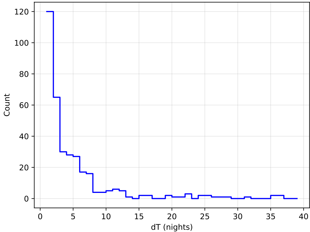
internal_u_expt38_nscale1.0v3.4_10yrs all bands: DD:WFD Delta Nights Histogram
