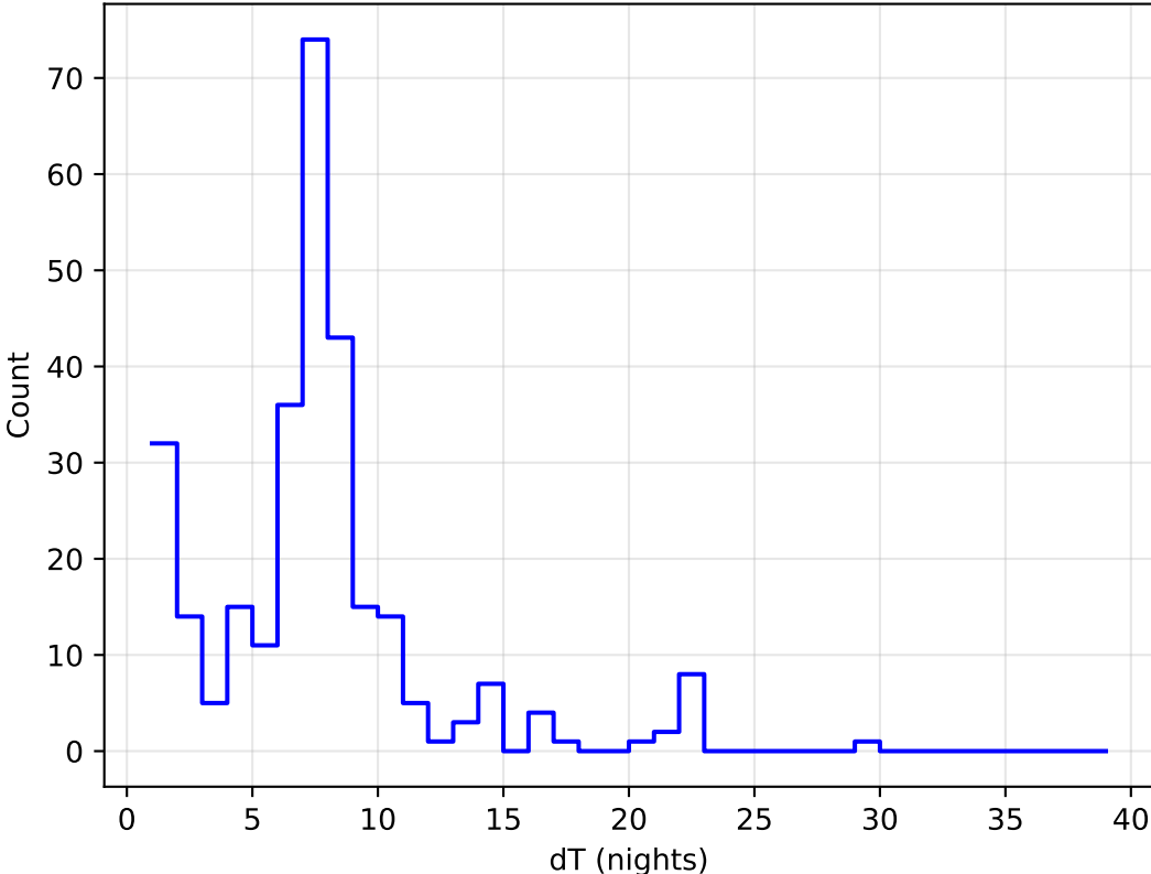
internal_u_expt38_nscale1.0v3.4_10yrs all bands: DD:EDFS Delta Nights Histogram
