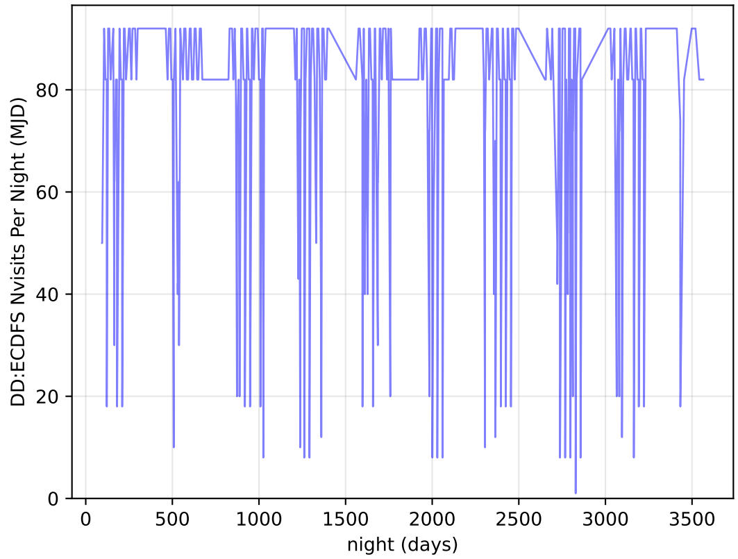
internal_u_expt38_nscale1.0v3.4_10yrs all bands: DD:ECDFS Nvisits Per Night
