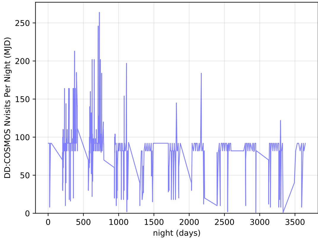
internal_u_expt38_nscale1.0v3.4_10yrs all bands: DD: COSMOS Nvisits Per Night
