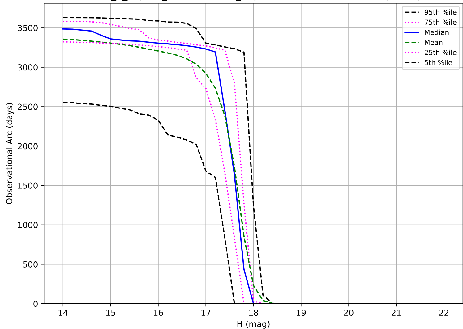
internal_u_expt38_nscale0.9v3.4_10yrs: Observational Arc Length Trojan
