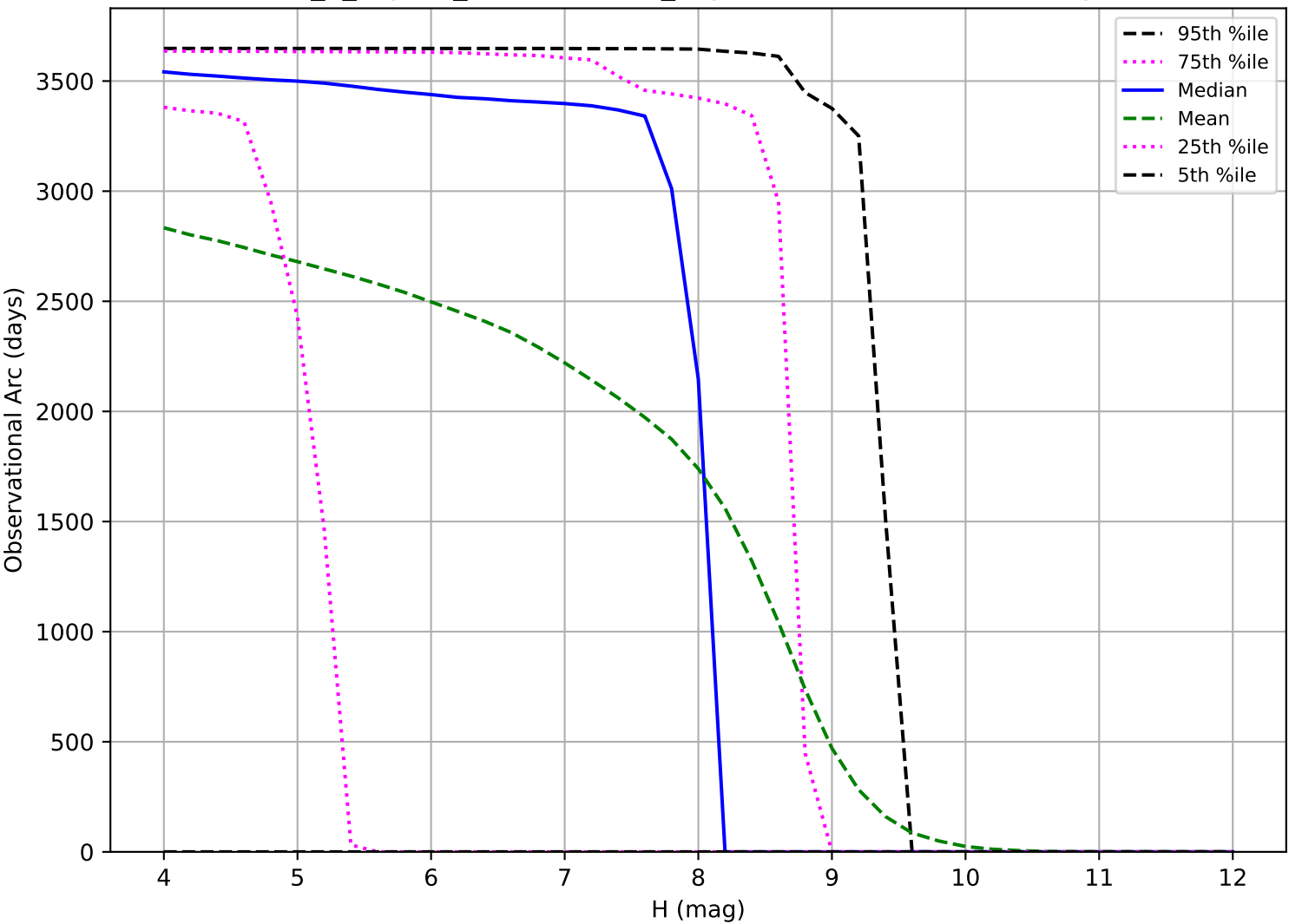
internal_u_expt38_nscale0.9v3.4_10yrs: Observational Arc Length TNO
