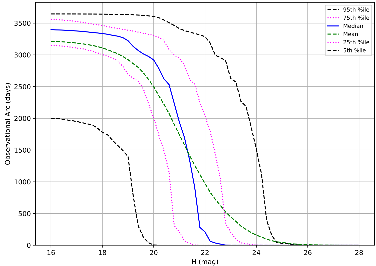
internal_u_expt38_nscale0.9v3.4_10yrs: Observational Arc Length PHA
